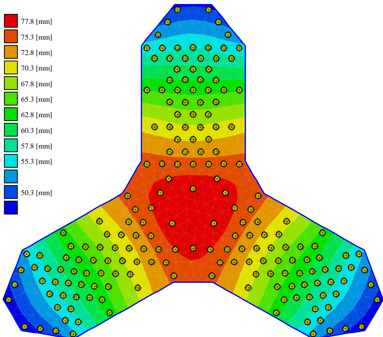
Figure 7-7 Settlement using the method "Hyperbolic Function for Load-Settlement Curve"
