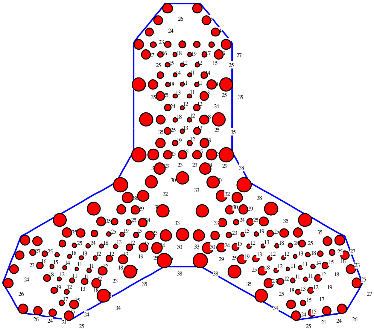
Figure 7-16 Pile load [MN] using the method "Given Load-Settlement Curve"
