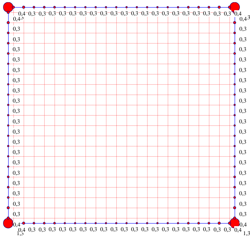
Figure 2-22 Contact pressures [MN/m 2 ] - LPR - Max. q = 10.3 [MN/m 2 ]
