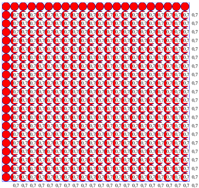
Figure 2-25 Pile loads Ph [MN]
