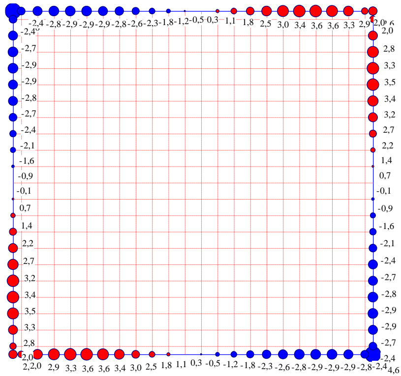
Figure 2-24 Contact pressures [MN/m 2 ] – NPRD - Max. q = 3.6 [MN/m 2 ] at the edge
