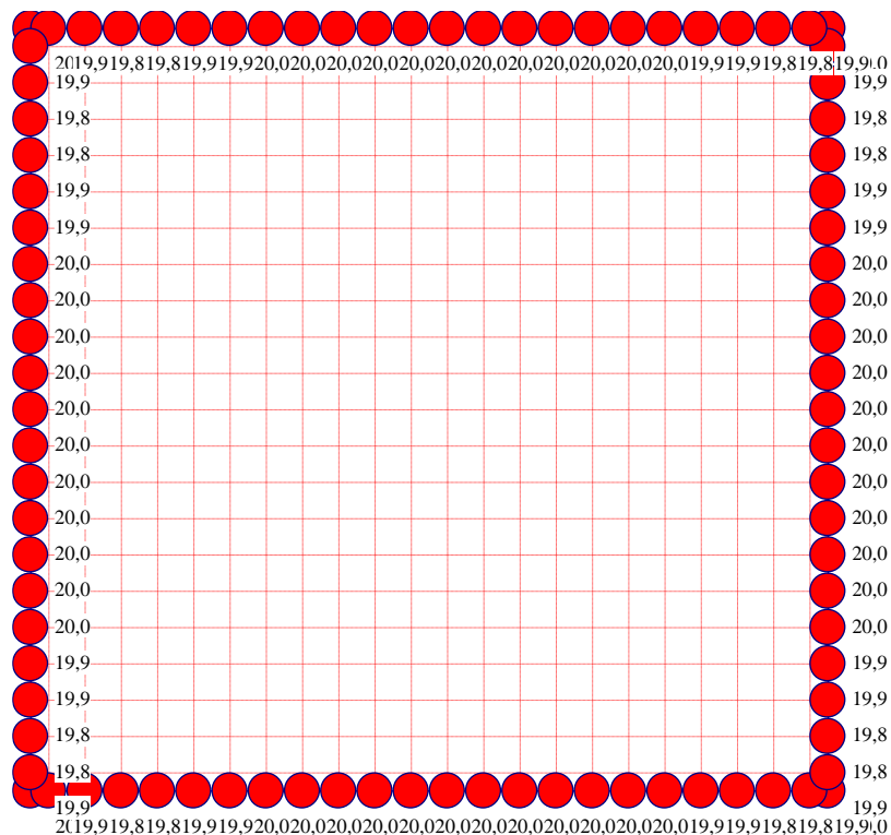
Figure 2-17 Contact pressures [MN/m 2 ] - NPRH - Max. q = 20 [kN/m 2 ] at the edges
