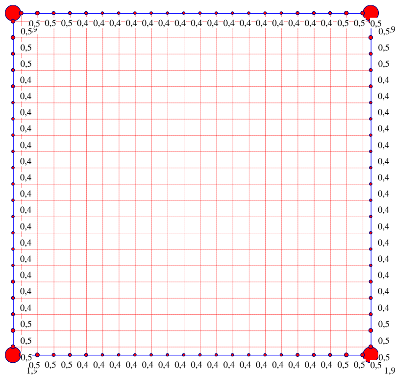
Figure 2-23 Contact pressures [MN/m 2 ] - NPRH - Max. q = 1.9 [MN/m 2 ] at the edge
