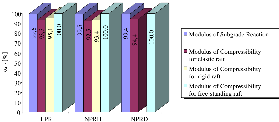
Figure 2-39 Bearing factors \alpha_{kPP} [%]
