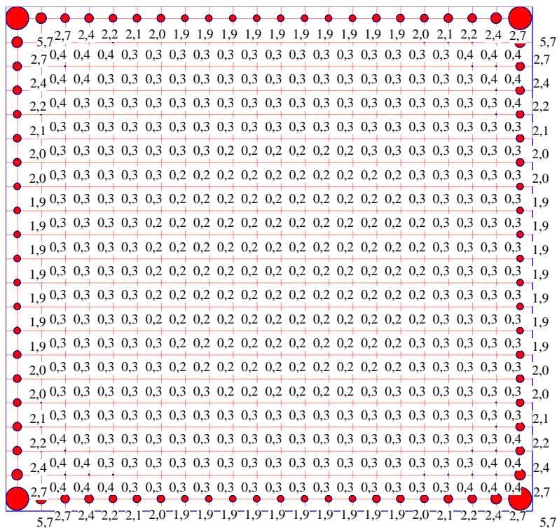
Figure 2-32 Pile loads Ph [MN] - LPR
